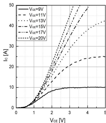
Fig 2. Typical output characteristic ( T_{vj}=175^{\circ}\text{C} )
