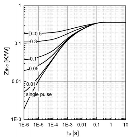
Fig 14. Transient thermal impedance of IGBT
